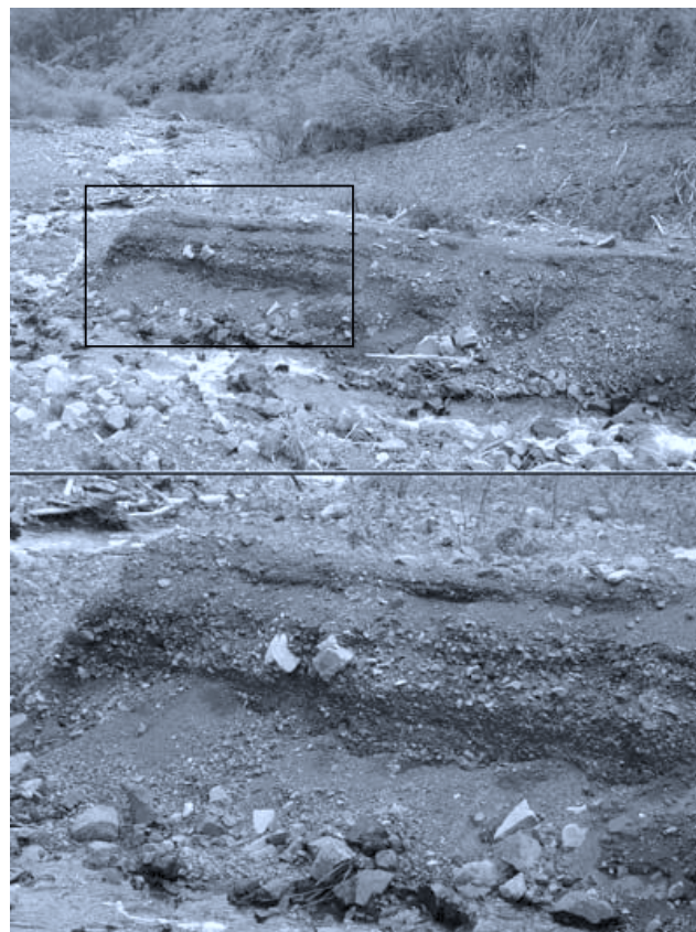
Figure 8 – Confluence between the second true-right tributary and the Tamaki trunk channel (top) showing cut banks of up to 6 m height with detail of the sheet deposits (bottom), probably deposited during the 2004 flood.
