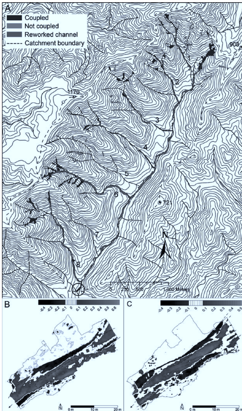
Figure 7 – (A) Areas of recent erosion and reworked channel within the Tamaki River catchment (contour lines at 20 m intervals) and their connectivity (coupled or not) to the study reach (circled); scour and fill (in m) at the study reach (B) between November 2007 and January 2008 and (C) between January and May 2008.
