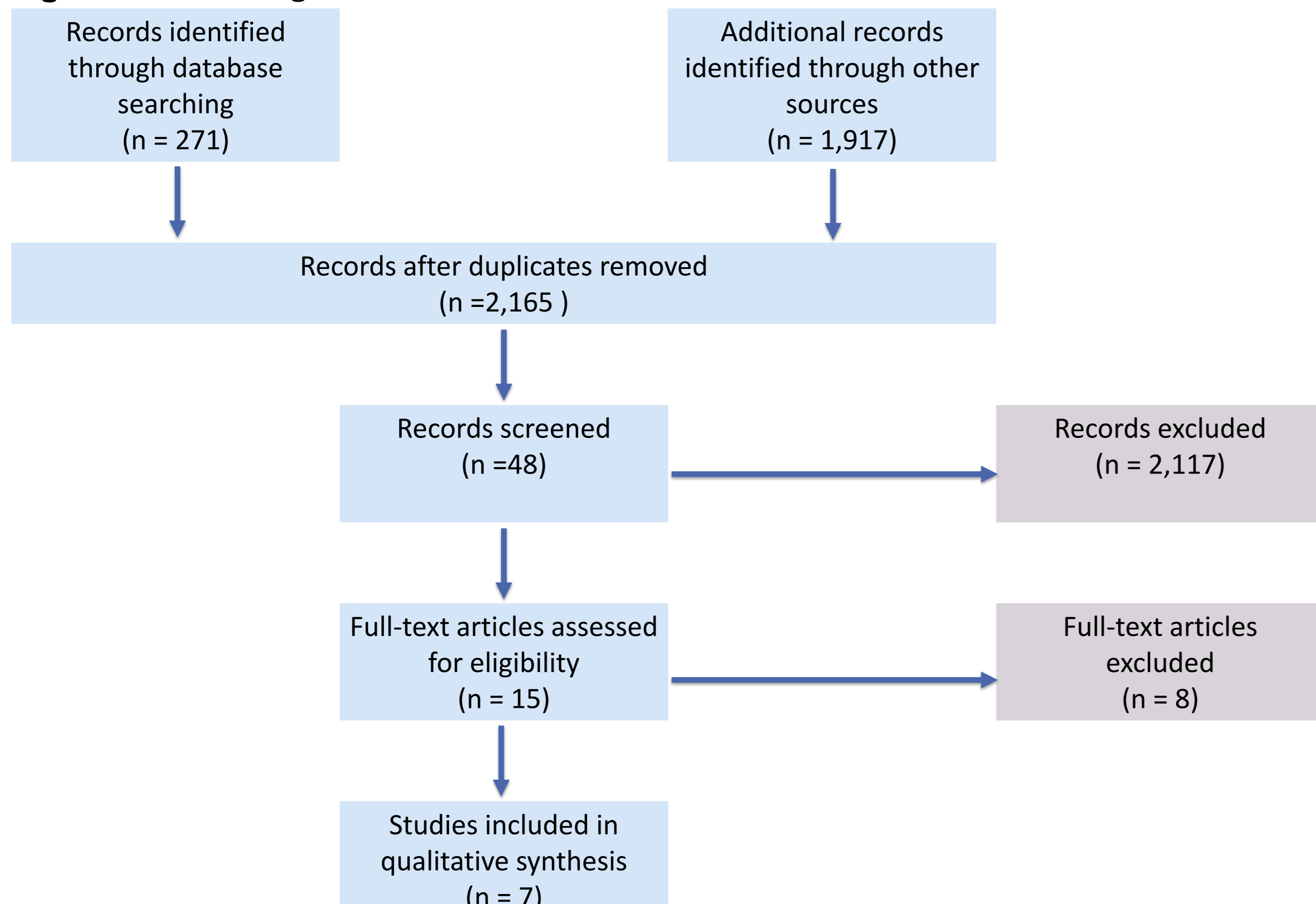
Figure 3: PRISMA Diagram
