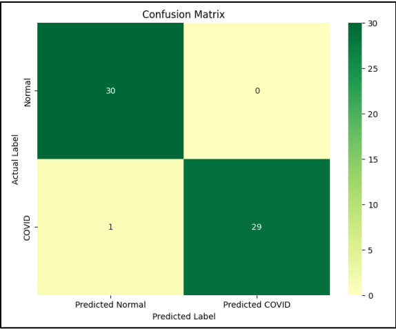
Figure 1 Confusion Matrix
