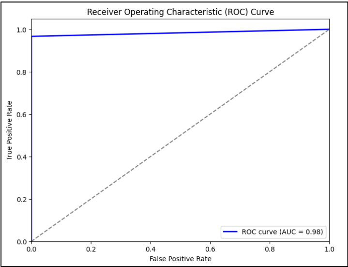
Figure 3 ROC Curve
