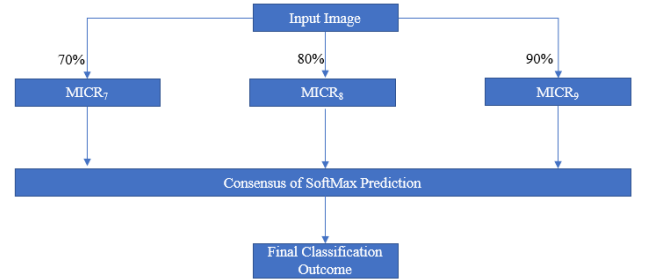
Fig. 4: Majority voting ensemble approach used
