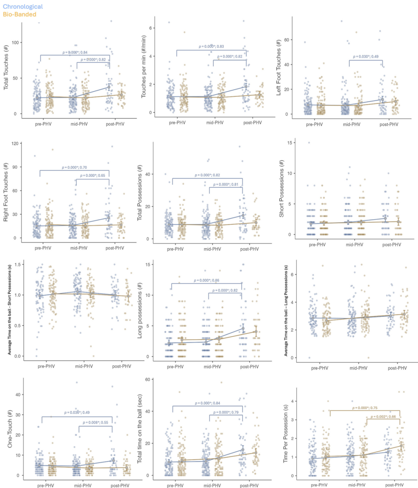
Fig. 3. Estimated marginal mean differences (mean ± SD with 95 % confidence intervals) in technical characteristics between chronological and bio-banded formats across biological maturity groups. Statistically significant differences between groups are highlighted ( p -value; Cohen's- d ).
