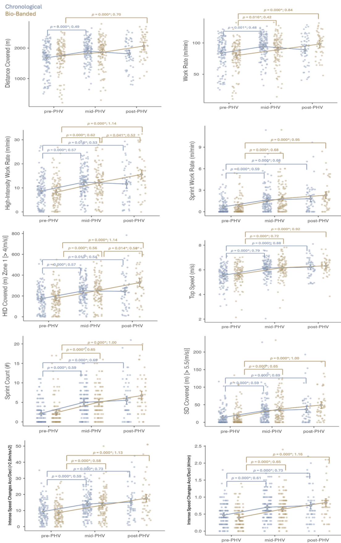
Fig. 2. Estimated marginal mean differences (mean \pm SD with 95 % confidence intervals) in physical characteristics between chronological and bio-banded formats across biological maturity groups. Statistically significant differences between groups are highlighted ( p -value; Cohen's- d ).
