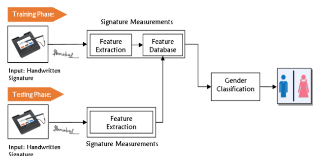
Fig. 1. Proposed architecture model for gender classification
