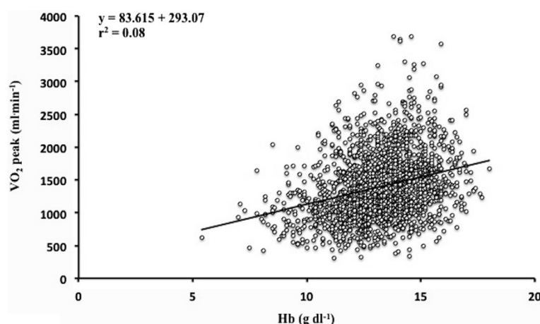
Figure 1 Linear regression between unadjusted \dot{V}O_2 peak ( \text{ml min}^{-1} ) and haemoglobin concentration ( [\text{Hb}] ), n = 1,774 .
