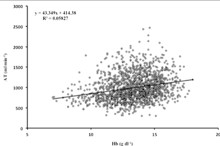
Figure 2 Linear regression between unadjusted oxygen uptake at anaerobic threshold (AT) ( \text{ml min}^{-1} ) and haemoglobin concentration ( [\text{Hb}] ), n = 1,631 .
