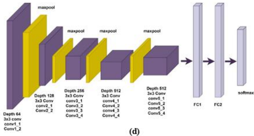
Figure 8. Architectural Diagrams of Pretrained Convolutional Neural Networks Used for Feature Extraction from Grad-CAM Attention-Enhanced Inputs: (a) ResNet50, (b) Xception, (c) VGG16, and (d) VGG19.
