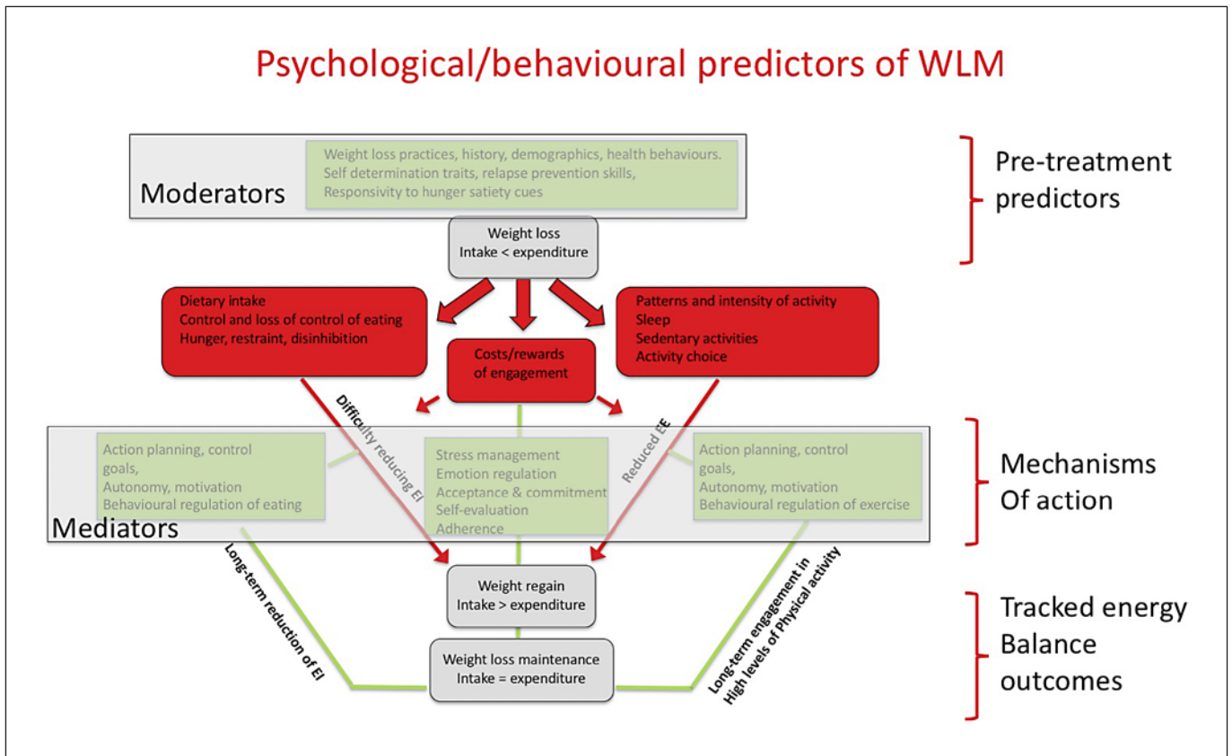
Fig. 3. Schematic adaptation of the NIH Working Group Report framework for maintenance of weight loss illustrating how pre-treatment predictors and mechanisms of action of behaviour change interventions relate to compensatory changes in the components of energy intake (EI) and energy expenditure (EE). At present, moderators, mediators of energy balance behaviours and
